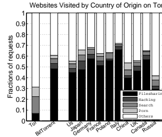
Figure 7: Distributions of the categories of websites visited by Tor users per country of origin. Tor represents the overall distribution of requests for all Tor users (not necessarily traced). BitTorrent represents the overall distribution of requests for traced Tor users. The other bars represent the same information but per country of origin. BitTorrent users on Tor visit significantly more Hacking websites and significantly less Search and Porn than regular Tor users.
